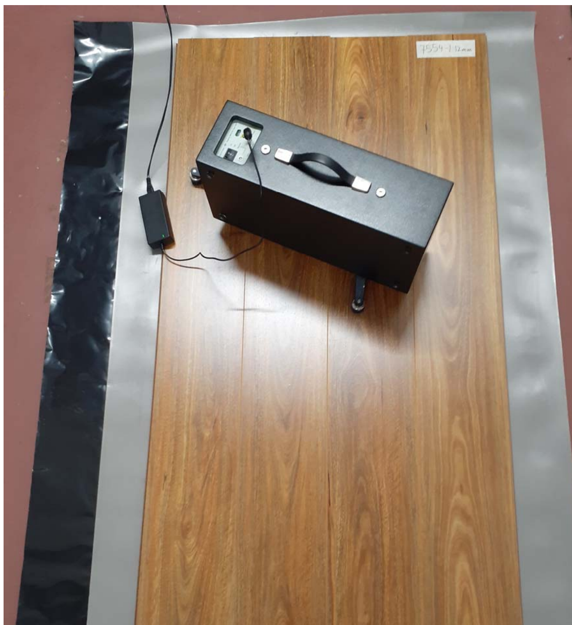
Figure 2. Image of testing configuration - '14 mm Oak' with 'Aqua Defend' underlay on base floor
