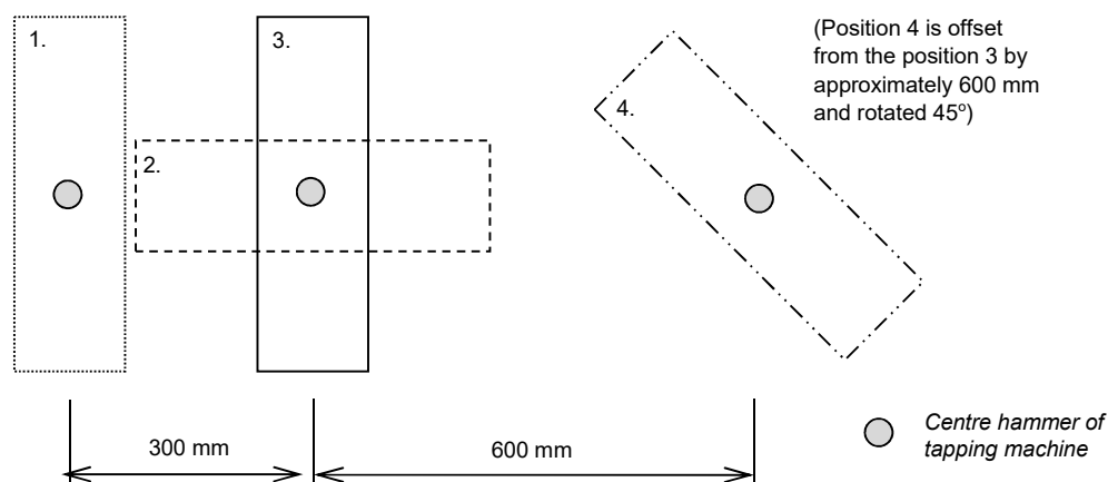
Figure 1. Tapping machine test orientations
